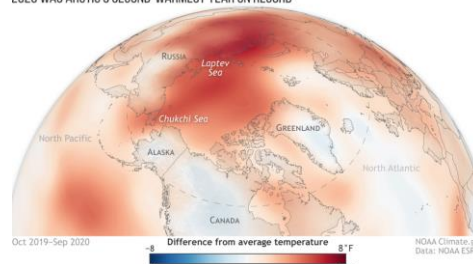
2020 WAS ARCTIC'S SECOND-WARMEST YEAR ON RECORD
